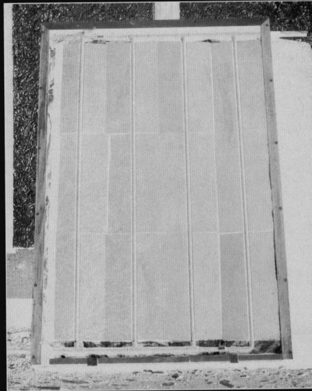
Fig. 4: The completed clip fin model solar collector, shown being made on the following pages.
