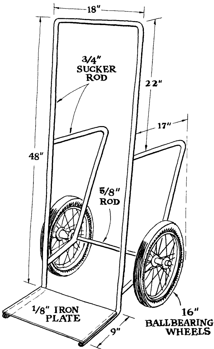
Dimensions for our homestead cart.
