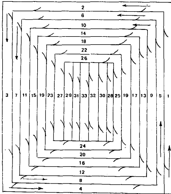
Fig. 45 - Ploughing continuously round and round the field
