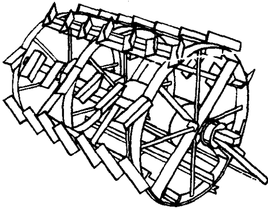
Fig. 97 - Puddling roller (with concrete ballast), Madagascar
