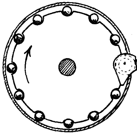
Fig. 113 - Horizontal plate seed distribution system
