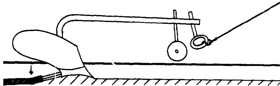
Fig. 52 Incorrect pitch adjustment: The wheel lifts off the ground and the heel piece presses too hard into the furrow bottom
