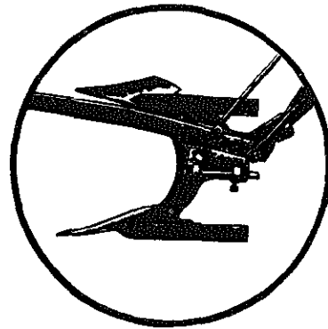
Detail of the pivoting system and locking by lever
