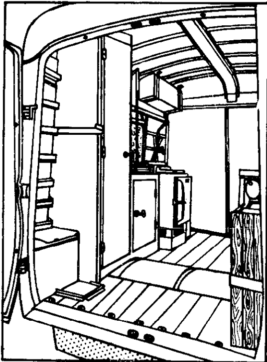
Fig. 178 - MALI service van accommodation section
