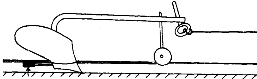
Fig. 51 Incorrect pitch adjustment: The wheel presses too heavily on the ground and the heel piece is up in the air
