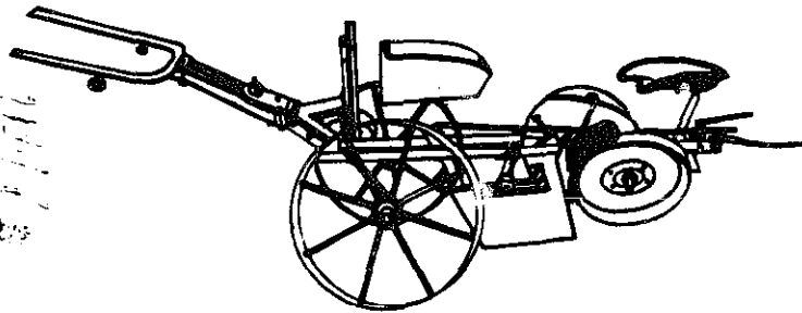
Fig. 115 - Transplanting implements
