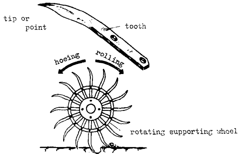
Fig. 129 - Tip and supporting wheel of pull type rotary hoe.
