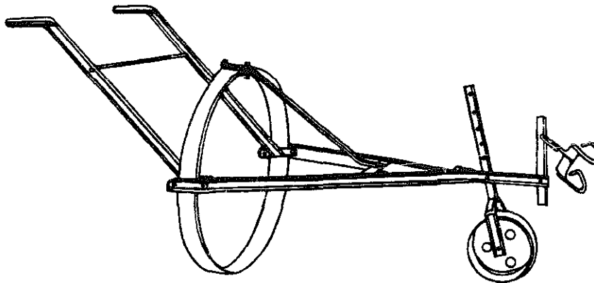
Fig. 147 - Sketches of various types of ground-nut lifter blades
