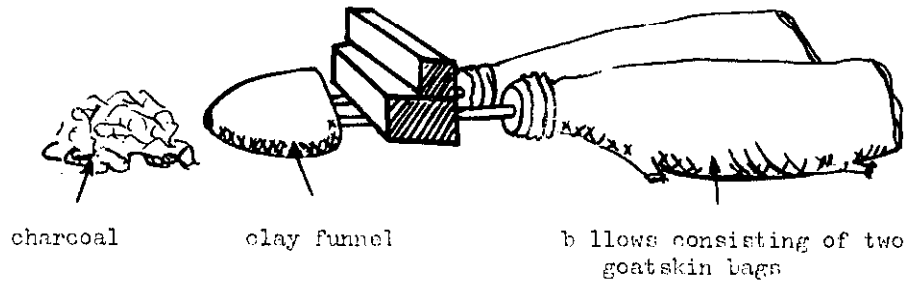
Fig. 175 - Sketch of a Nigerian artisan's traditional forge
