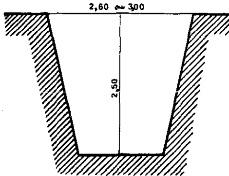
Fig. 10 Section of a silage trench
