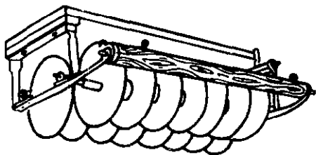
Fig. 100 "Carret del favo" Spanish disc harrow
