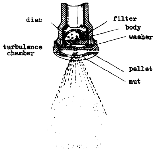
Fig. 132 - Section of plain turbulence chamber nozzle
