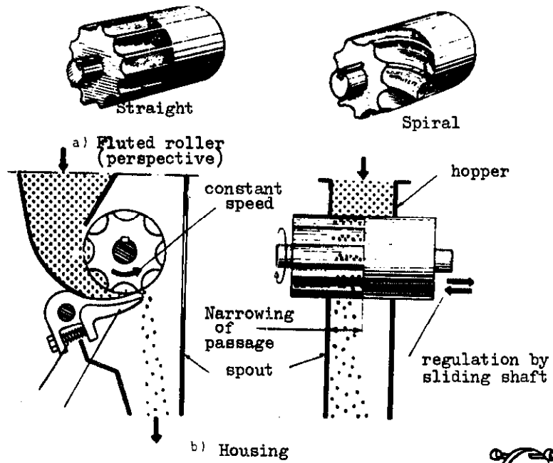
Fig. 106 - Fluted roller feed system
