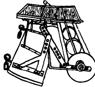
Fig. 98 - Type of puddling machine made in Spain
