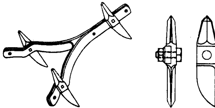
Fig. 76 - Reversible teeth for spike tooth harrows
