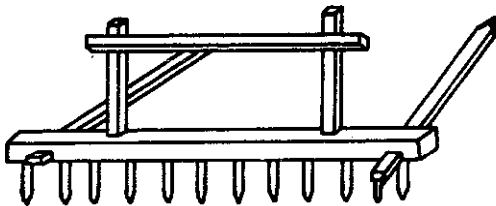
Fig. 89 - Comb-harrow
