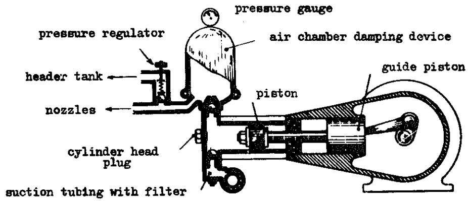
Fig. 137 - Layout of a piston pump with pressure regulator
