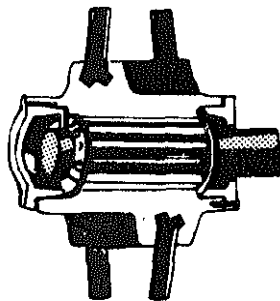
roller bearings
