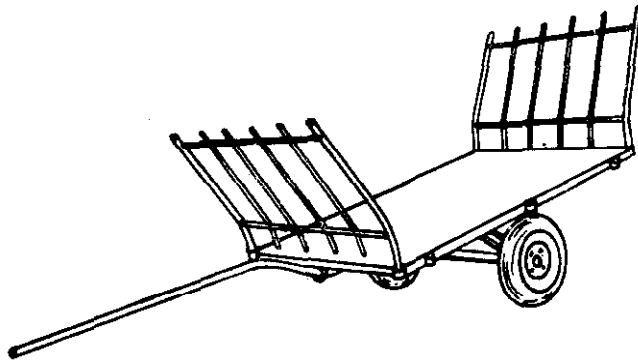
Fig. 158 - 1,000 kg farm wagon "AFRICA No.2 type", with pole for ox draught.
