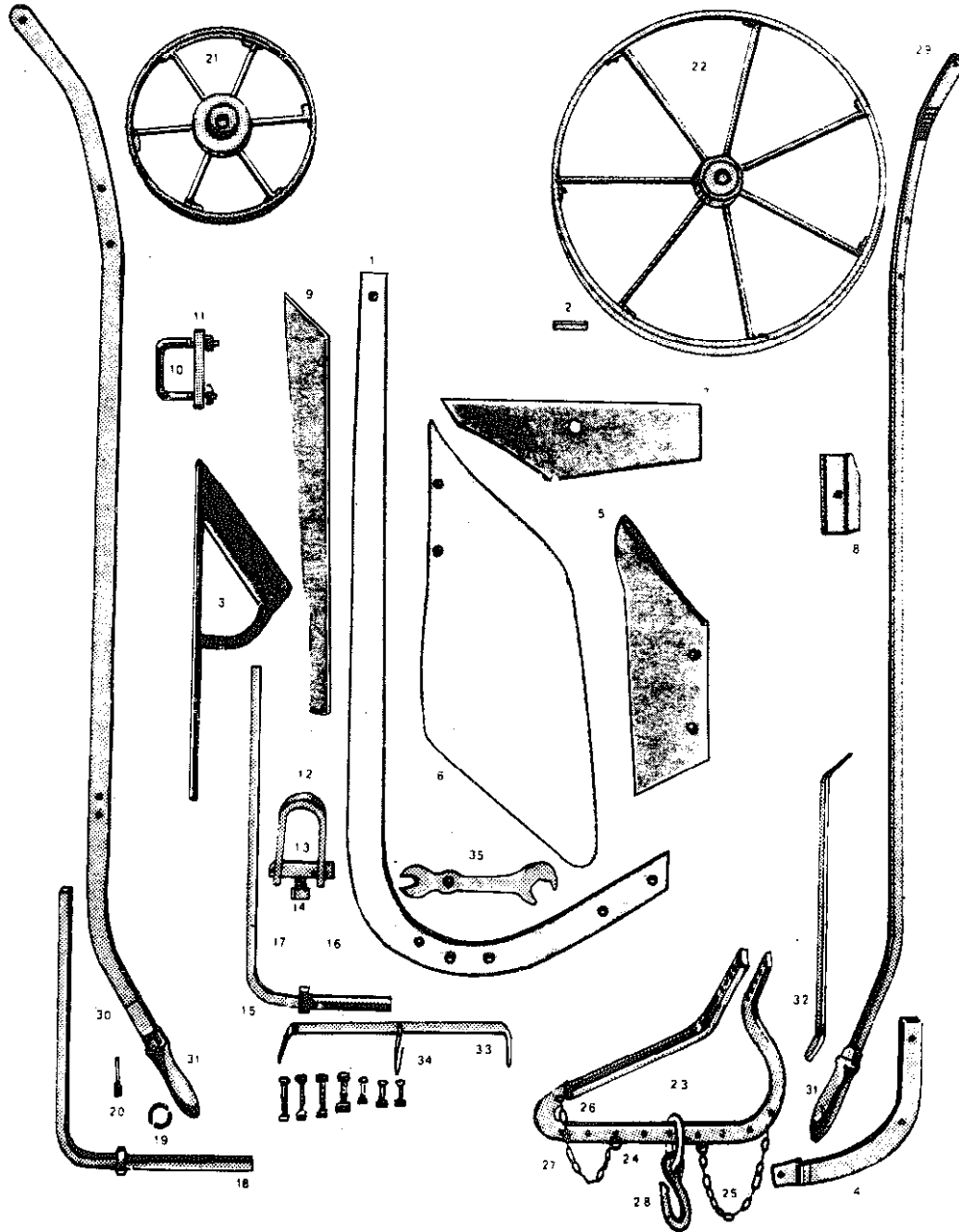
Fig. 47 - The parts of a plough
