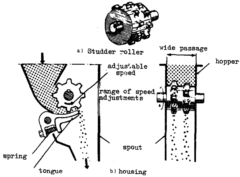
Fig. 107 - Studder roller feed system
