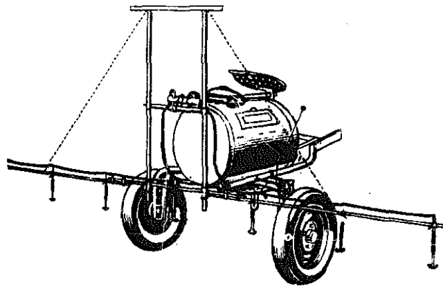
Fig. 141 - Animal draught sprayer
