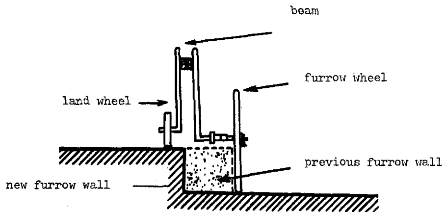
Fig. 55 - Positions of the supporting wheels during ploughing (plough viewed from behind)
