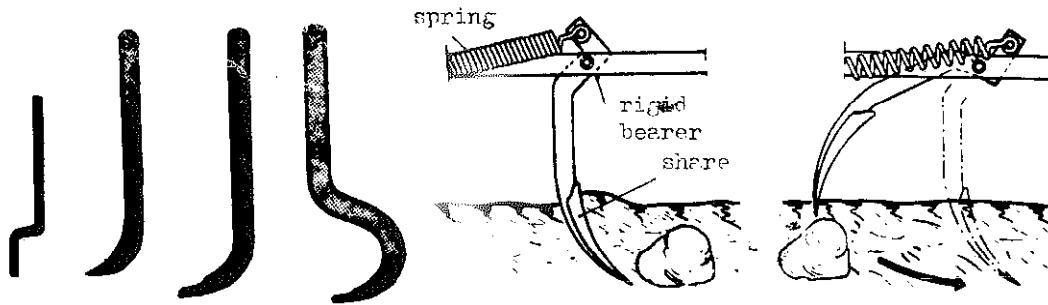
Fig. 69 - Retractable rigid tine-spring loaded
