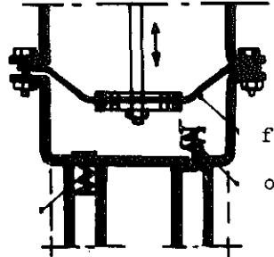
Fig. 135 Layout of a single membrane pump
