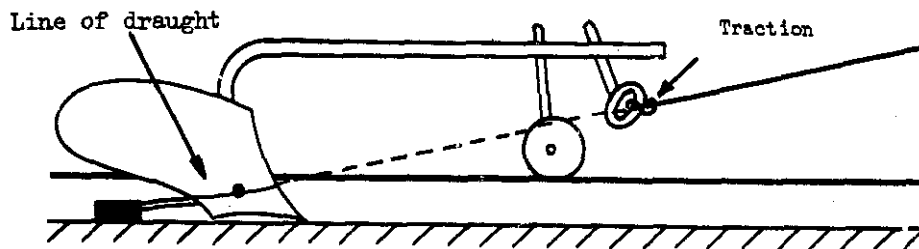
Fig. 53 Correct pitch adjustment: Heel piece sits on furrow bottom at the same level as the point of the share
