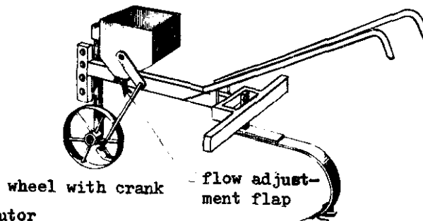
Fig. 121 -- Placement type distributor for fertilizer and insecticides
