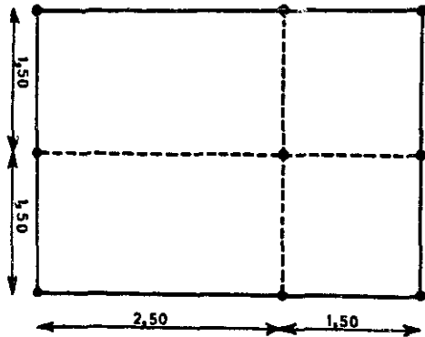
Fig. 3 - Plan of a cattleshed for two animals
