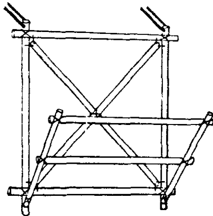
Sketch of cradle fitting
