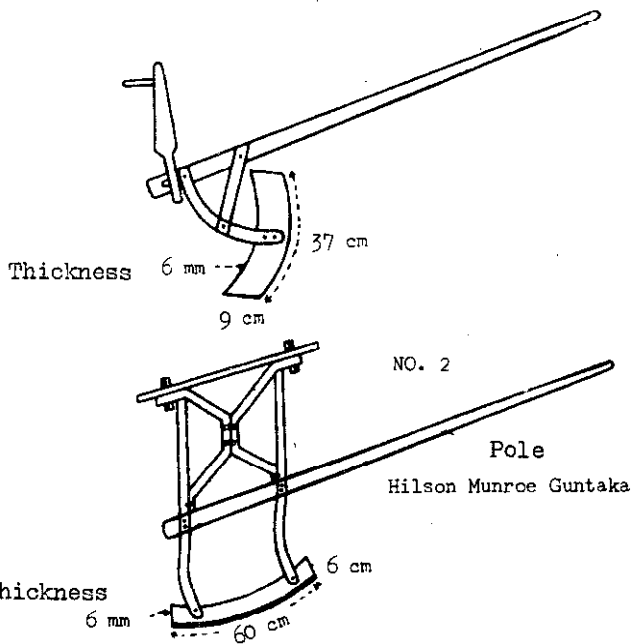
Fig. 151 - Improved "Guntakas" used in India
