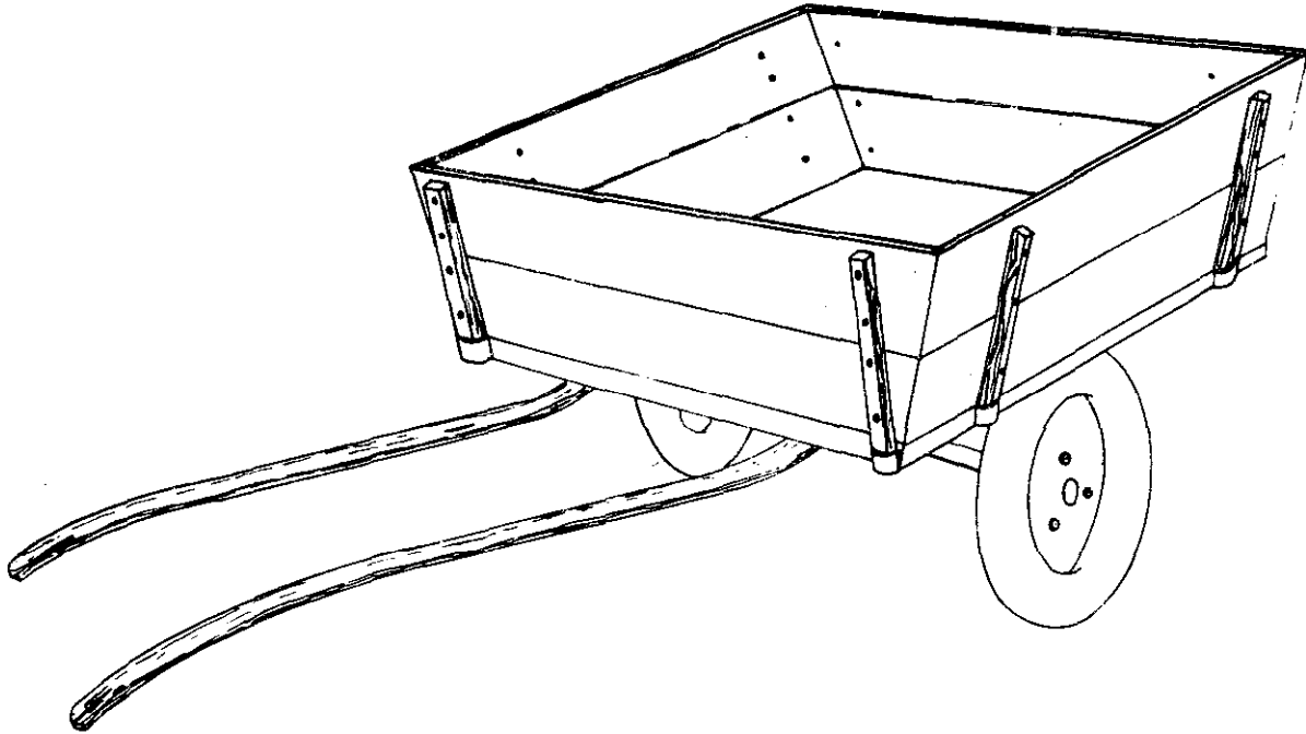
Fig. 157 - Donkey-cart with shafts (useful load 400 kg)
